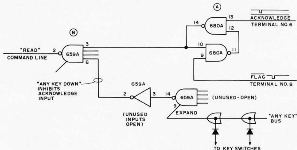
Fig. 5. Keyboard "Read" and Acknowledge logic.
