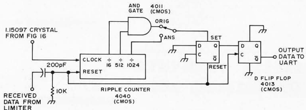
Fig. 18. Digital discriminator needs no adjustments or calibration.
