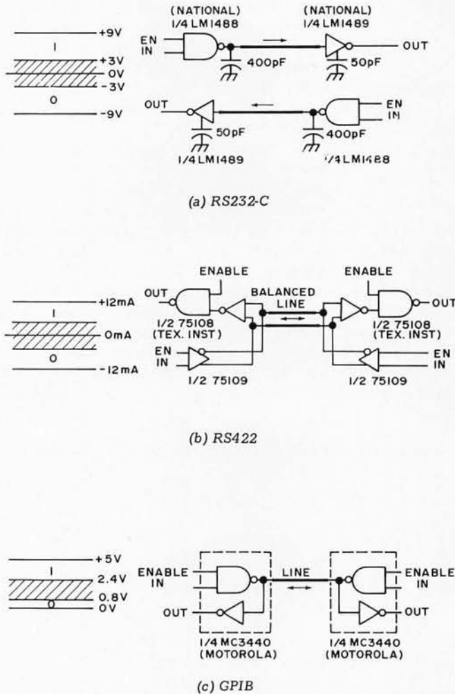
Fig. 7. Industrial interfaces for cable interconnections.
