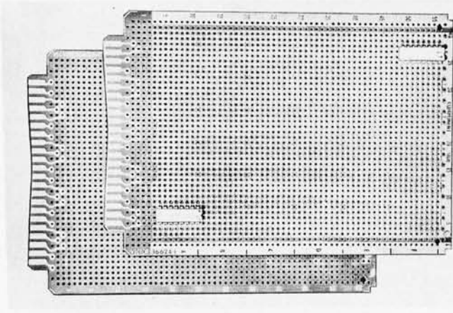
Edge connector configuration on Vector 3662A-6 Plugboard reduces insertion forces by 2-1/2 lbs.
